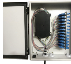
96 Port Wall Mount LIU
